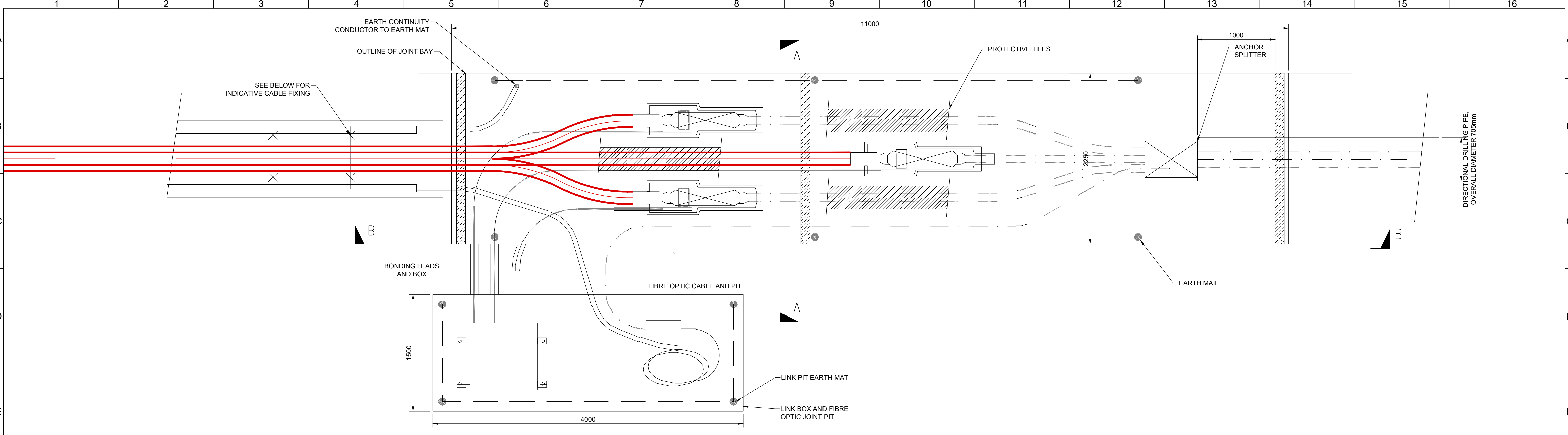
INDICATIVE TRANSITION JOINT BAY ARRANGEMENT SCALE 1:25
